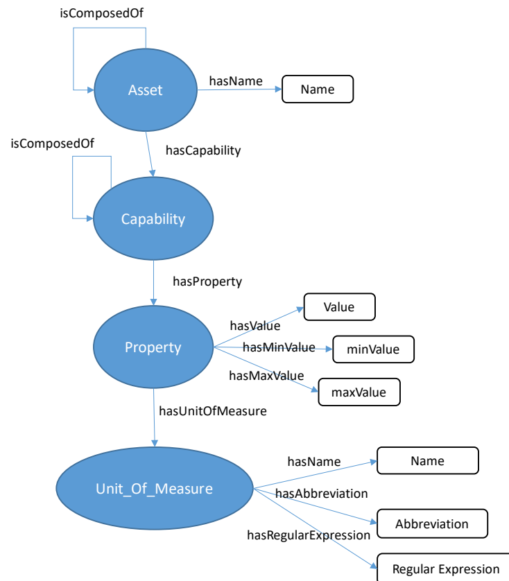
Figure 3: Fundamental ontology of Smart Factory Web
