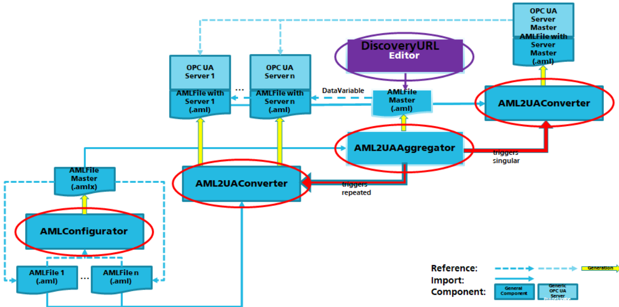
Figure 20: Extended AML2UA converter - Multi-level conversion
