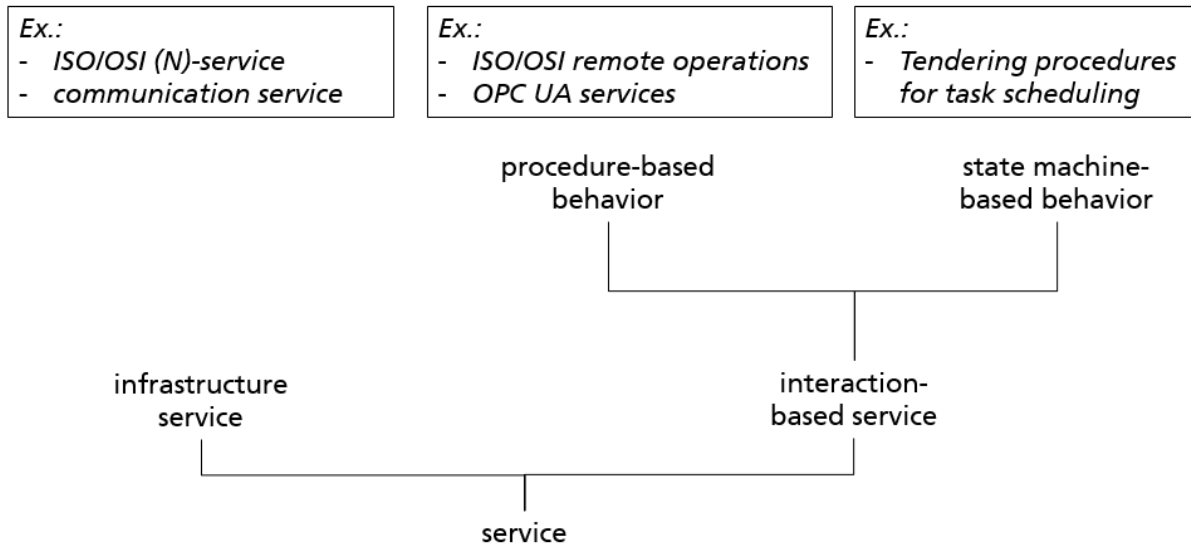
Figure 1: Basic classification of service types
