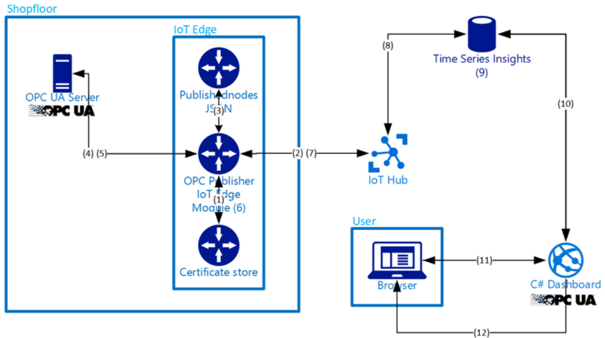
Figure 24: Secure Data Flow in MS Azure
